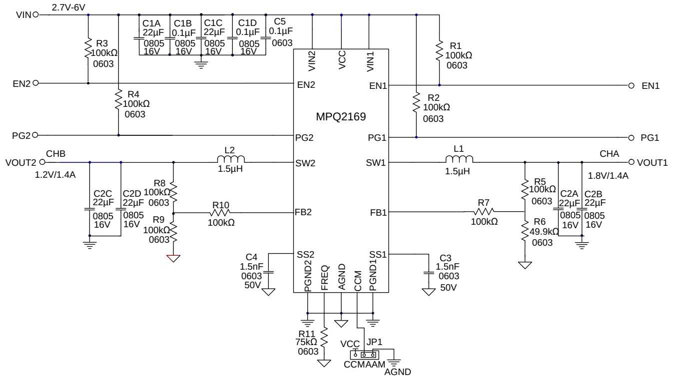
Figure 7: 1.4A/1.4A Application Circuit
