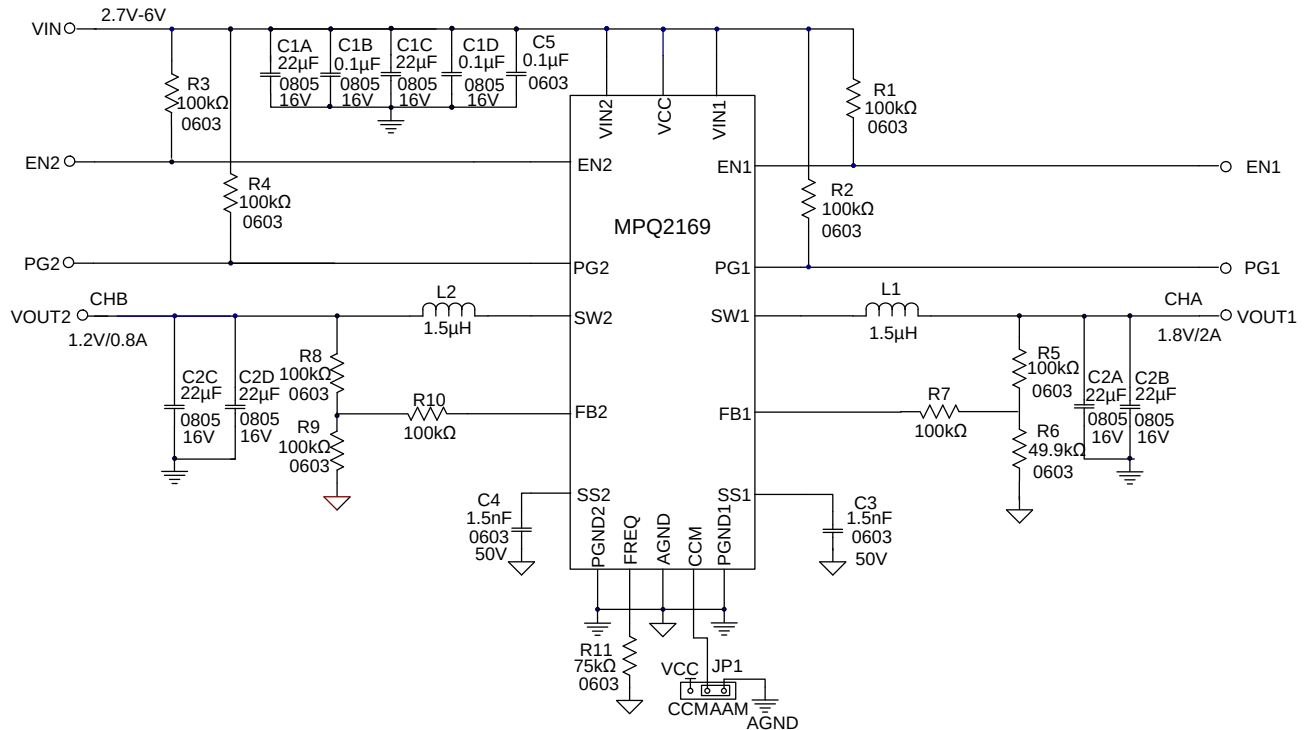
Figure 8 : 2A/0.8A Application Circuit
