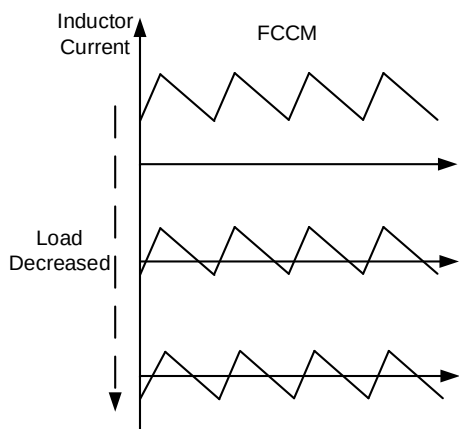
Figure 3: FCCM
