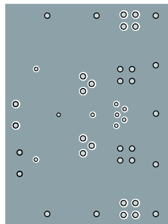
Mid-Layer 1
