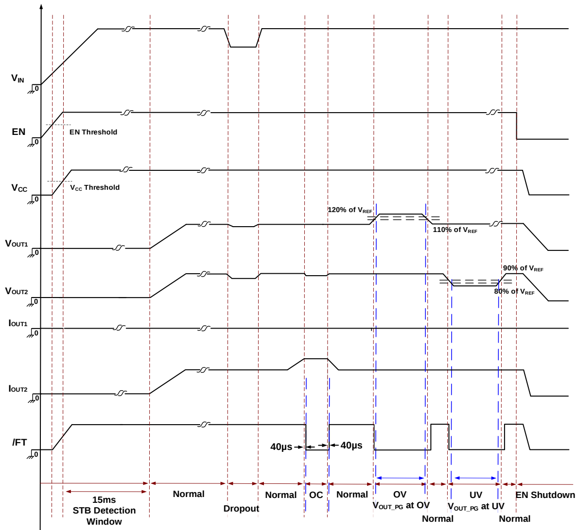
Figure 3: Timing Sequence
