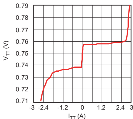
DDR3 Regulation
