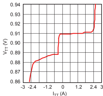
DDR2 Regulation
