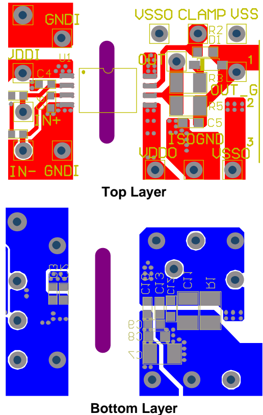
Figure 18: Recommended PCB Layout (21)
