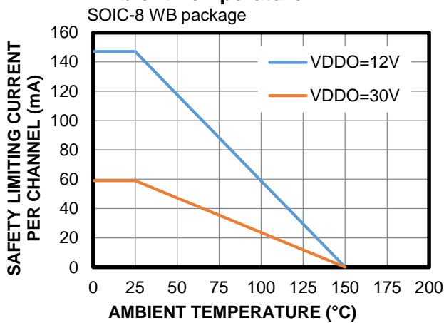
Safety Limiting Current vs. Ambient Temperature
