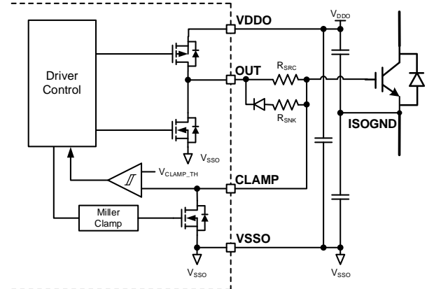
Figure 12: Active Miller Clamp
