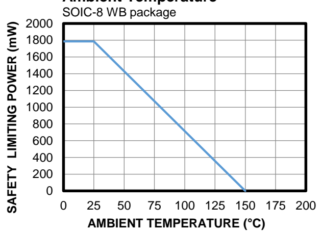
Safety Limiting Power vs. Ambient Temperature
