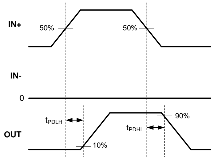
Figure 2: Non-Inverting Logic Propagation Delay
