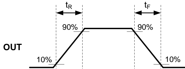
Figure 1: Output Rising and Falling Time
