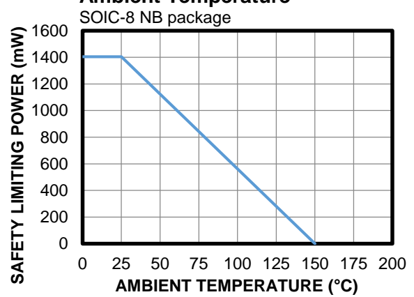
Safety Limiting Power vs. Ambient Temperature
