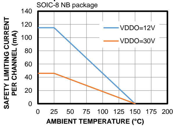
Safety Limiting Current per Channel vs. Ambient Temperature
