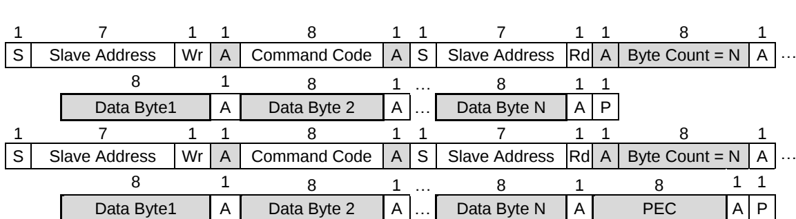
Figure 7: PMBus Message Format
