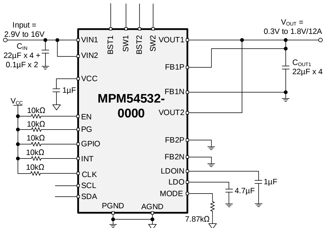
Figure 19: Typical Application Circuit (Dual-Phase Operation with Internal Divider)
