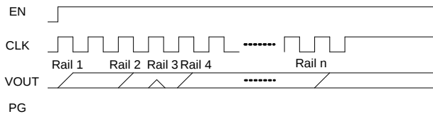
Figure 9: Soft Start during PMIC Error when CLK Does Not Pull Down (No CLK Pausing)
