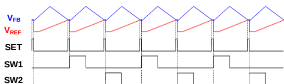
Figure 2: Buck 1/2 Interleaving for Dual-Phase Operation
