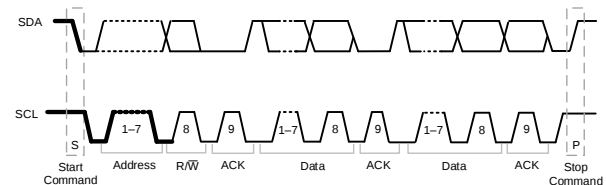
Figure 12: Complete Data Transfer
