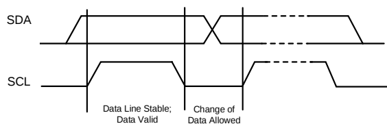
Figure 10: Bit Transfer on the I 2 C Bus
