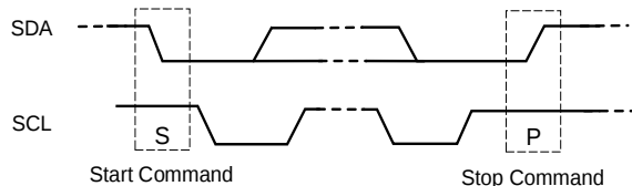
Figure 11: Start and Stop Commands
