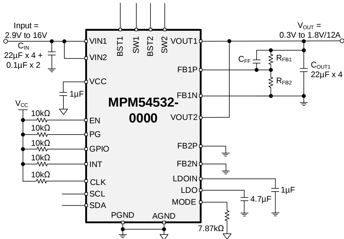
Figure 18: Typical Application Circuit (Dual-Phase Operation with External Divider)
