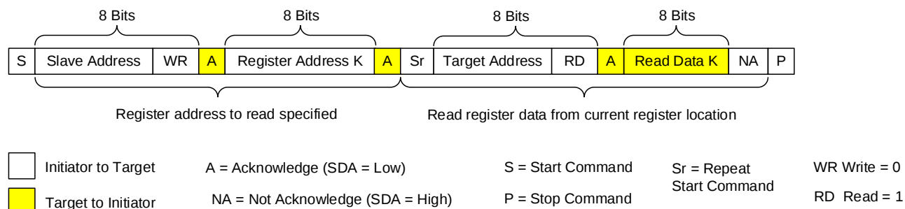
Figure 14: I 2 C Read Single Register Example
