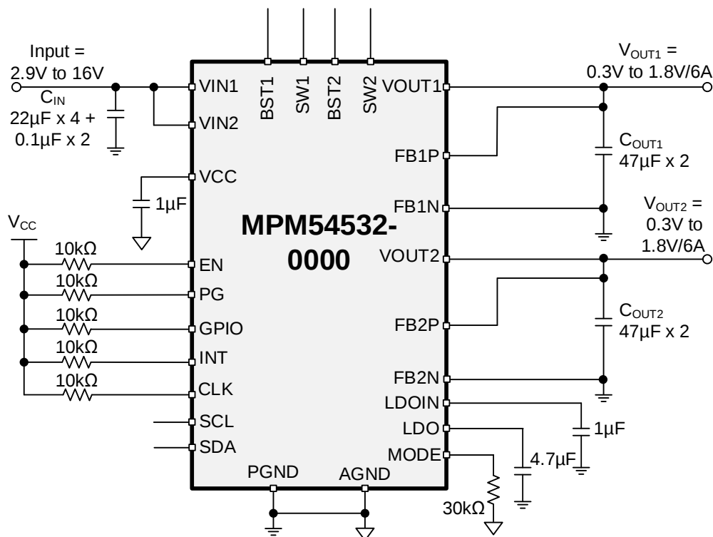
Figure 17: Typical Application Circuit (Dual-Output Operation with Internal Divider)
