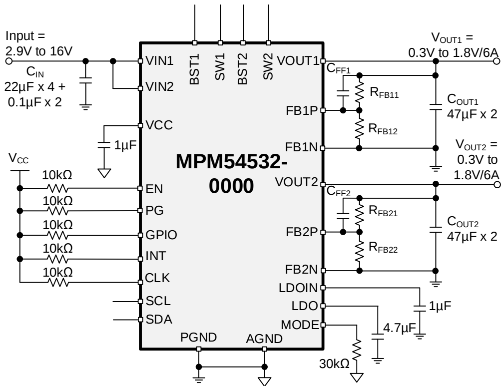
Figure 16: Typical Application Circuit (Dual-Output Operation with External Divider)
