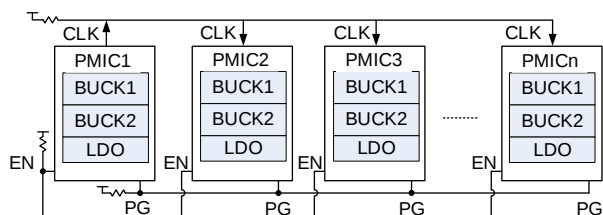
Figure 3: FLEX-Timer Sequence Control Connection
