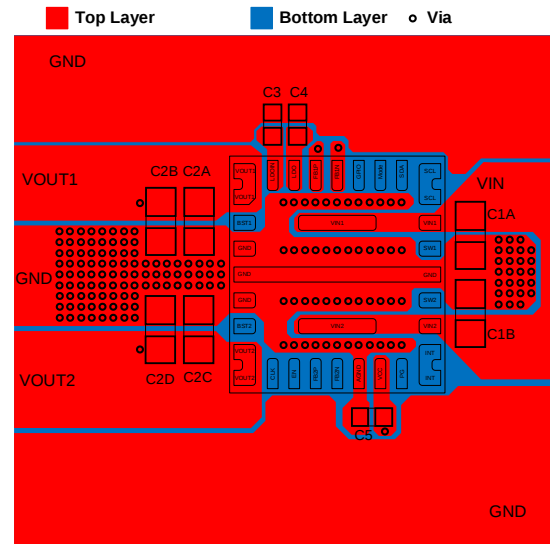
Figure 15: Recommended PCB Layout (Placement and Top Layer)
