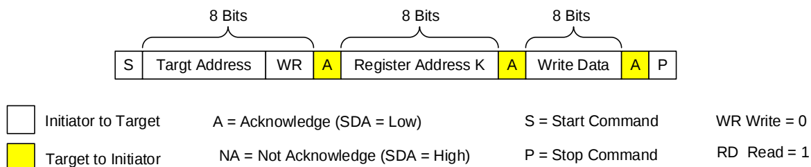
Figure 13: I 2 C Write Single Register Example
