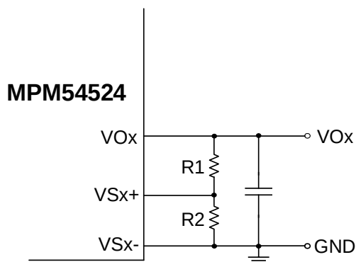
Figure 11: Feedback Network
