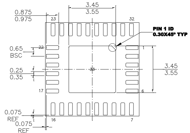
BOTTOM VIEW
