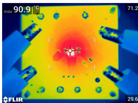
Thermal Rise I_{OUT} = 6A , T_A = 29.6^{\circ}C
