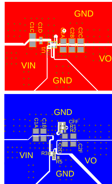
Figure 3: Recommended PCB Layout
