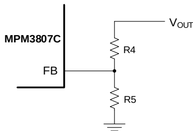
Figure 6: Feedback Network
