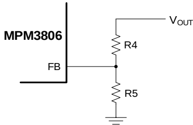
Figure 8: Feedback Network
