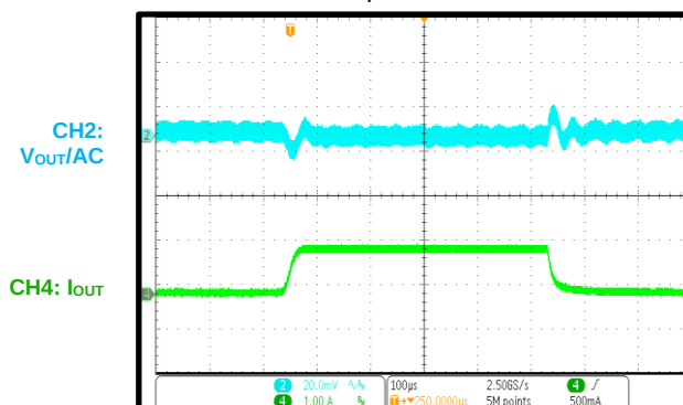
Load Transient
