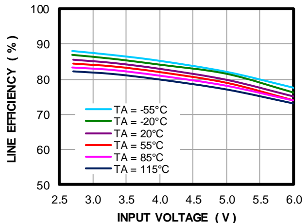
Line Efficiency
