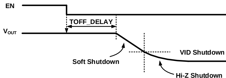
Figure 25: EN Soft-Off to Hi-Z Shutdown Level
