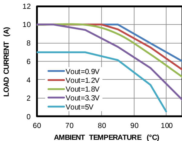
Thermal Derating
