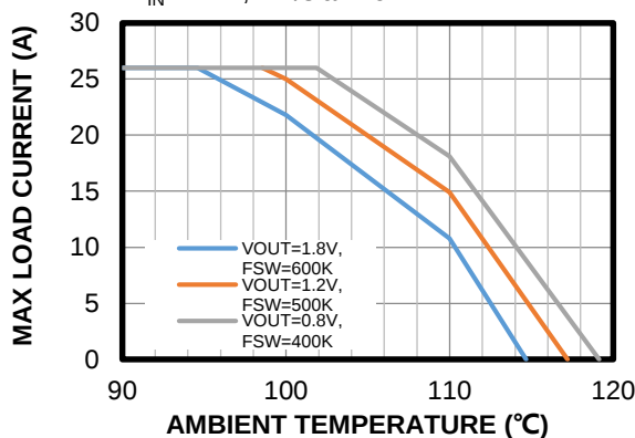
Thermal derating
