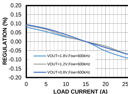
Load Regulation
