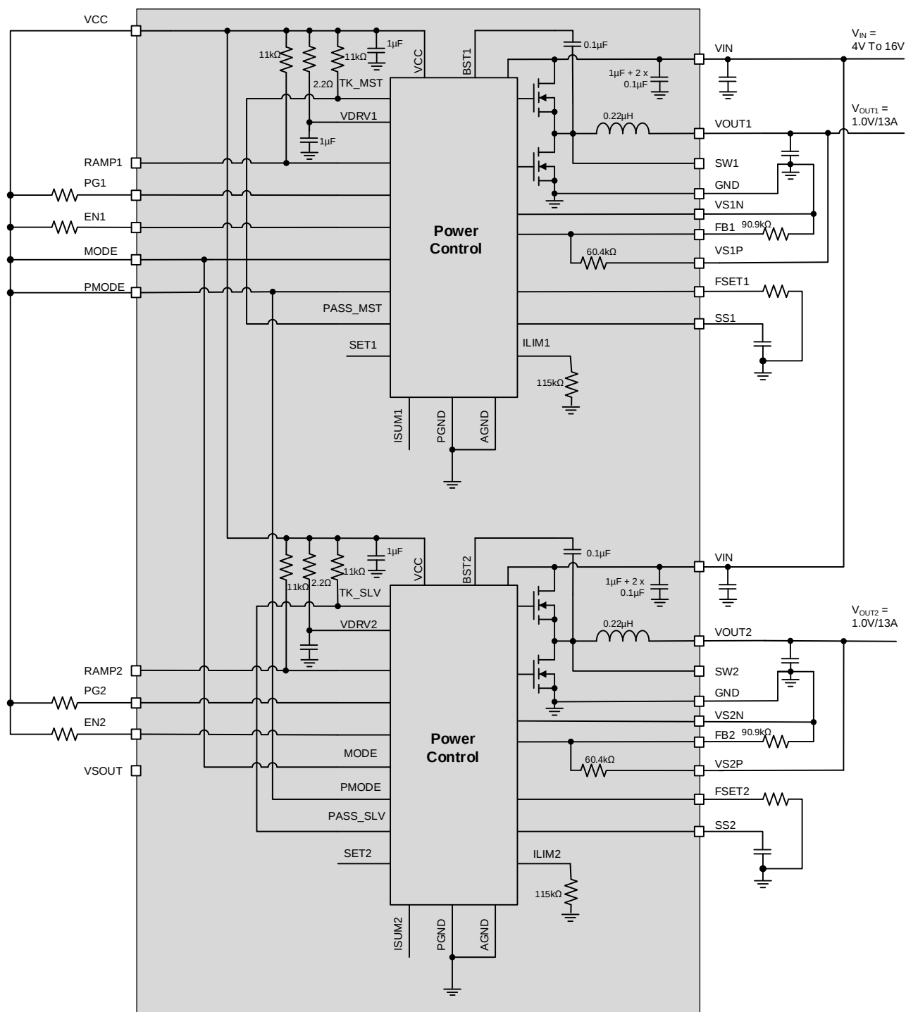
Figure 2: MPM3690-20A Functional Block Diagram
