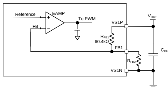
Figure 4: Feedback Circuit of the MPM3690-20
