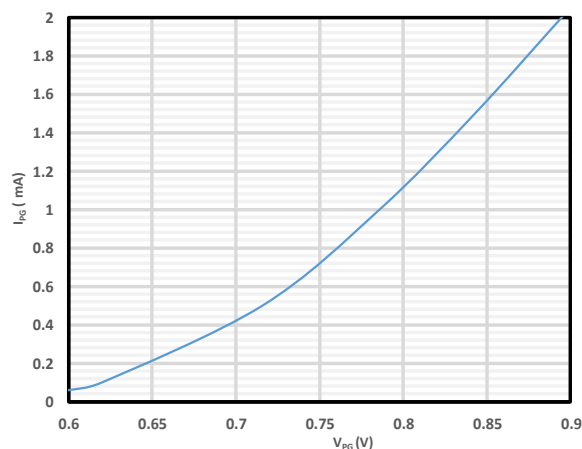
Figure 5: PG current vs. PG voltage
