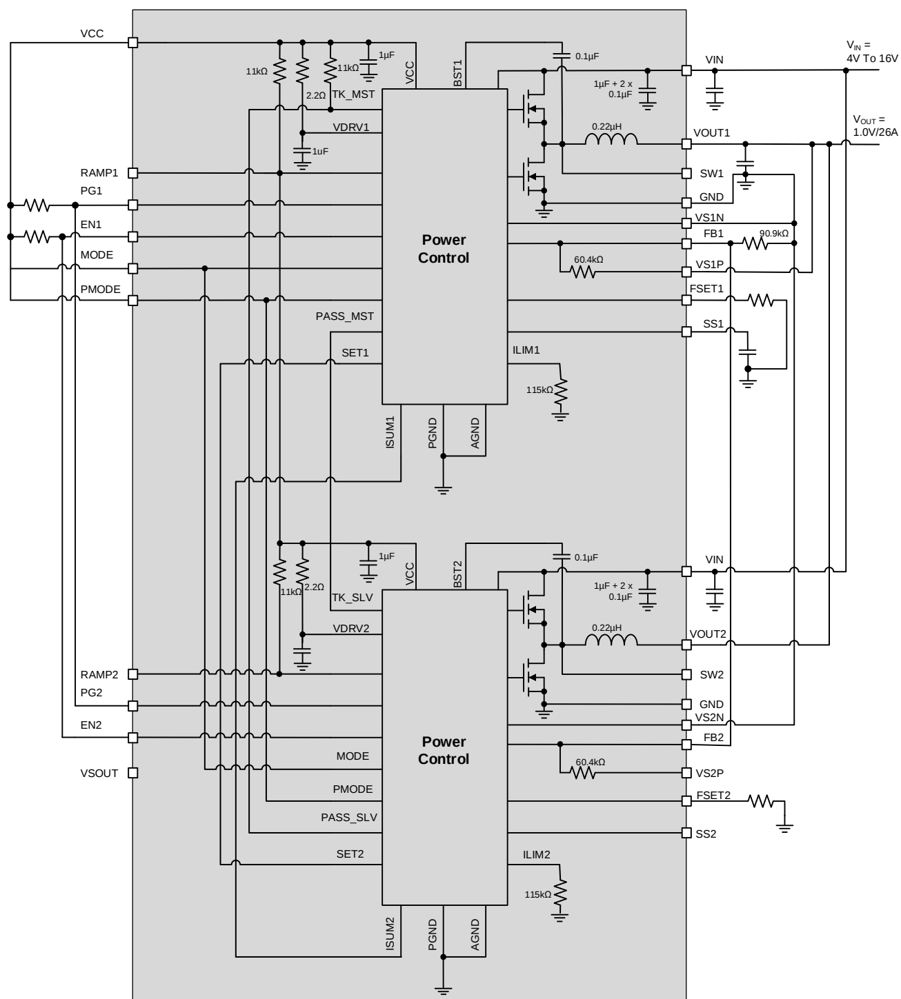
Figure 3: MPM3690-20B Functional Block Diagram
