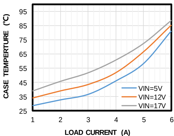
Case Temperature vs. Load Current
