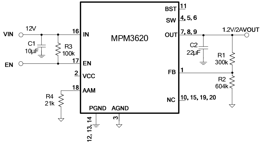
Figure 17. V_{OUT}=1.2V , I_{OUT}=2A
