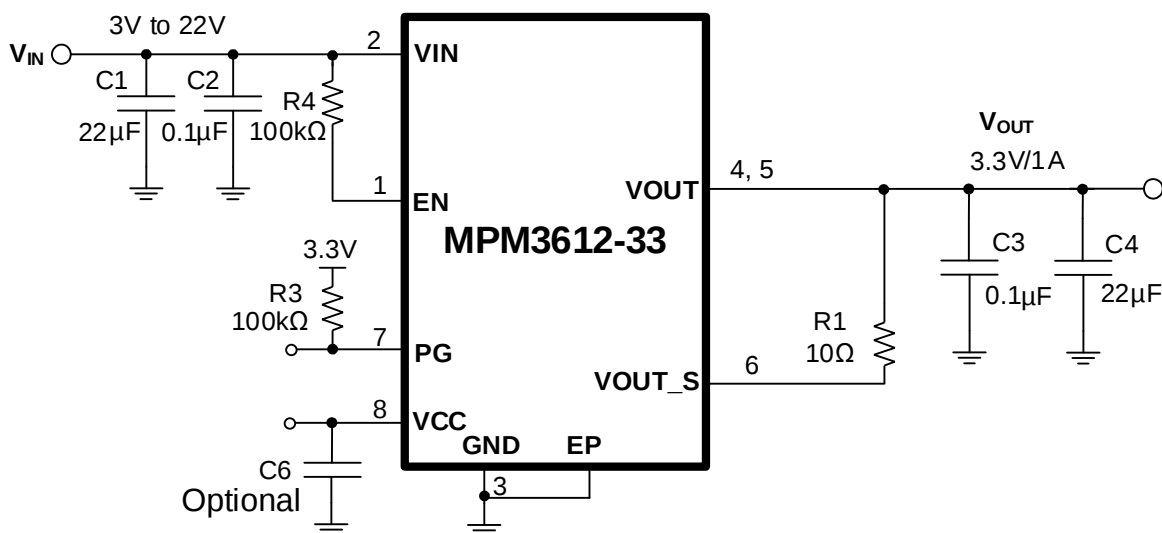
Figure 5: MPM3612-33 Typical Application Circuit
