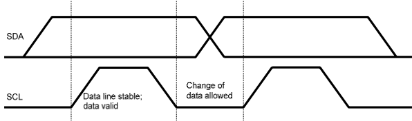
Figure 7: Bit Transfer on the I²C Bus
