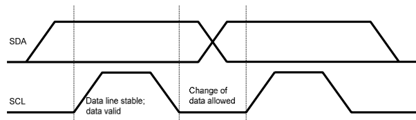
Figure 7: Bit Transfer on the I²C Bus
