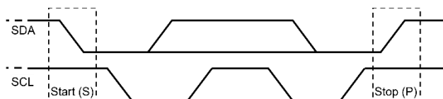
Figure 8: I²C Start and Stop Commands
