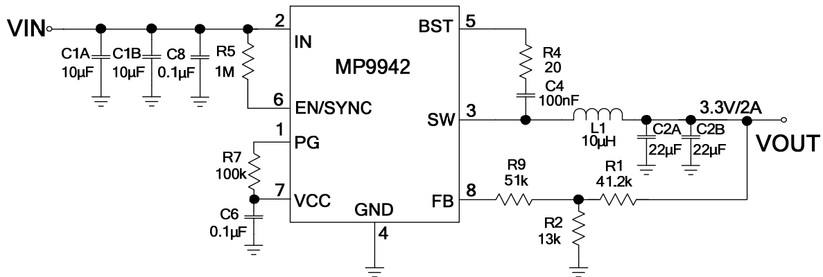
Figure 9: 12V IN , 3.3V/2A Output
