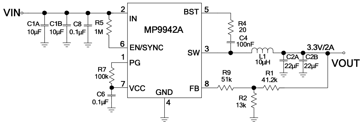
Figure 8: 12V IN , 3.3V/2A Output
