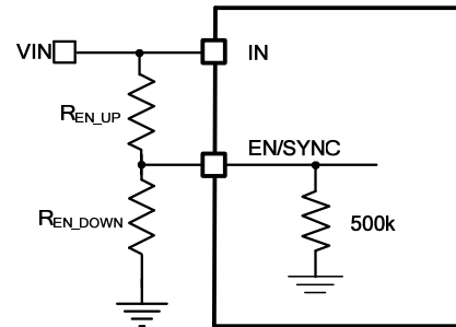
Figure 5: Adjustable UVLO using EN divider
