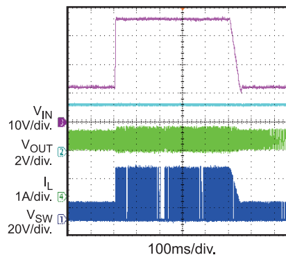
Load Dump
