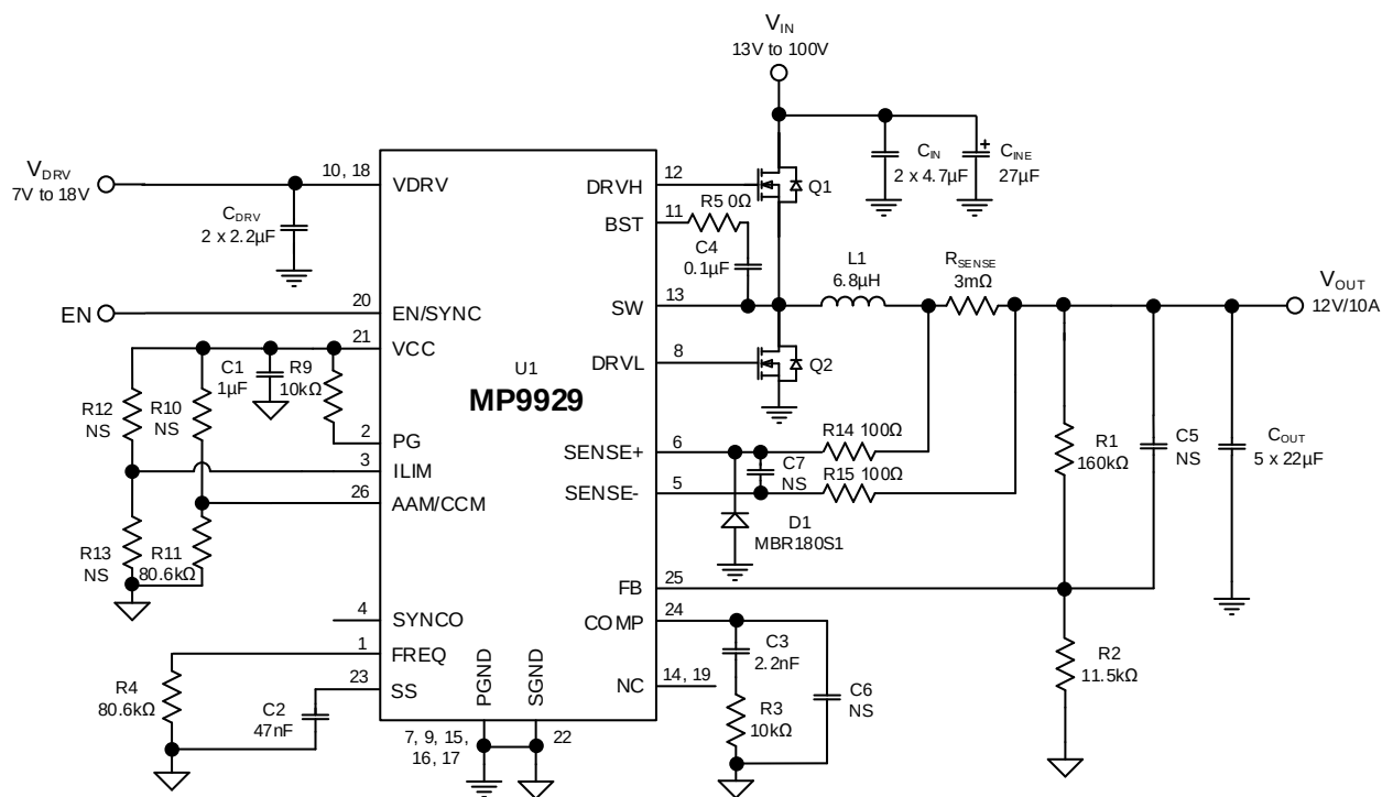
Figure 9: Typical Application Circuit (12V Output) (8)
