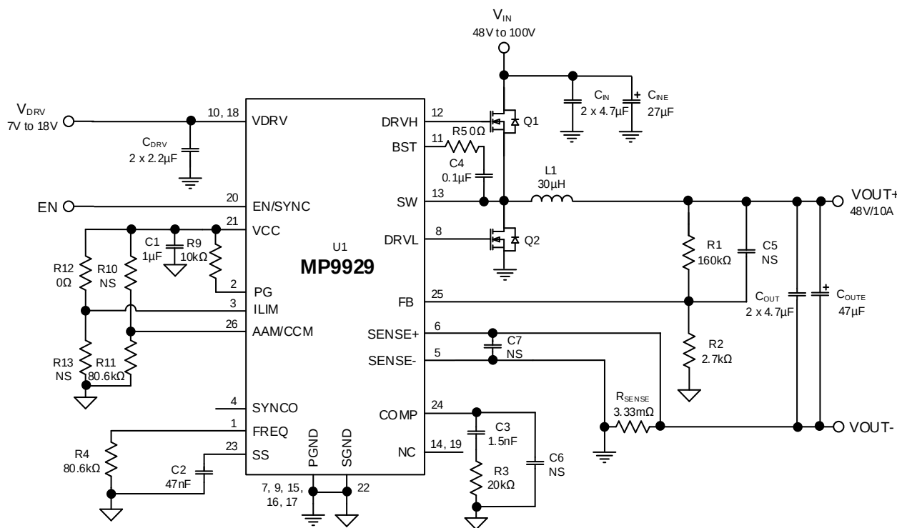
Figure 10: Typical Application Circuit (48V Output) (8)
