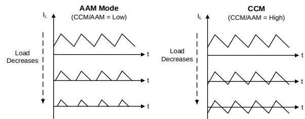
Figure 2: AAM Mode and CCM
