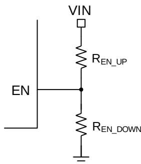
Figure 4: EN Resistor Divider
