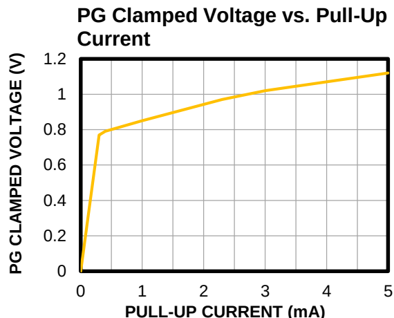
Figure 3: PG Clamped Voltage vs. Pull-Up Current
