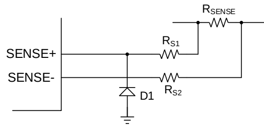
Figure 6: Negative Voltage Protection on SENSE+ and SENSE-
