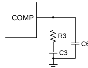
Figure 7: COMP External Compensation
