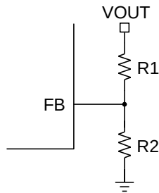
Figure 5: V_{OUT} Setting Resistor
