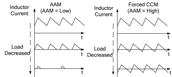
Figure 2: AAM and Forced CCM
