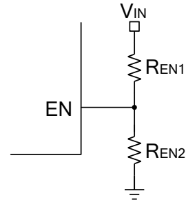
Figure 3: Enable Divider Circuit
