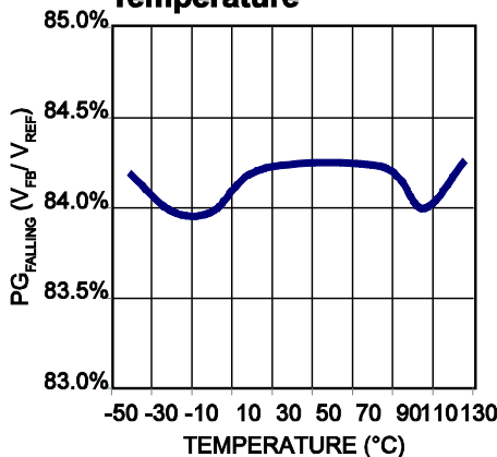
PG Falling Threshold ( V_{FB} Falling) vs. Temperature
