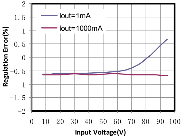
Line Regulation
