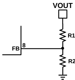
Figure 4: Feedback Network
