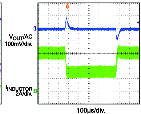
Load Transient Reponse I_{OUT} = 3A - 6A
