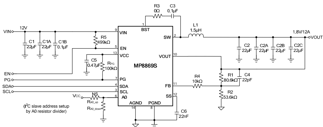
Figure 18: VIN = 12V, VOUT = 1.8V, IOUT = 12A
