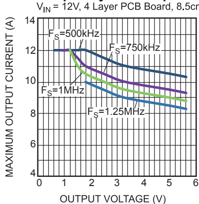
Output Current Derating vs. Frequency and Output Voltage V_{IN} = 12V , 4 Layer PCB Board, 8.5cmx8.5cm
