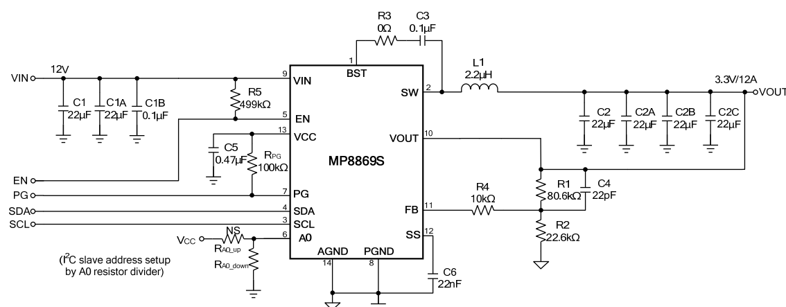
Figure 20: VIN = 12V, VOUT = 3.3V, IOUT = 12A
