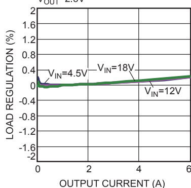
Load Regulation vs. Output Current V_{OUT}=2.5V
