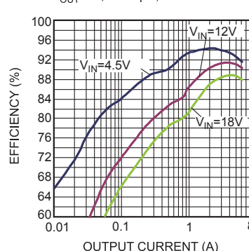
Efficiency vs. Output Current V OUT =1V, L=1.5µH, DCR=2.1mΩ
