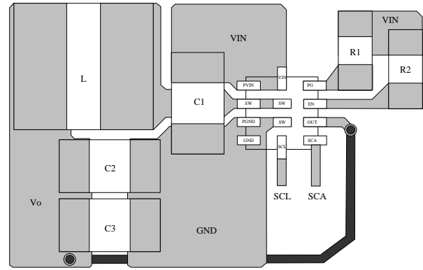
Figure 5: Recommended Layout
