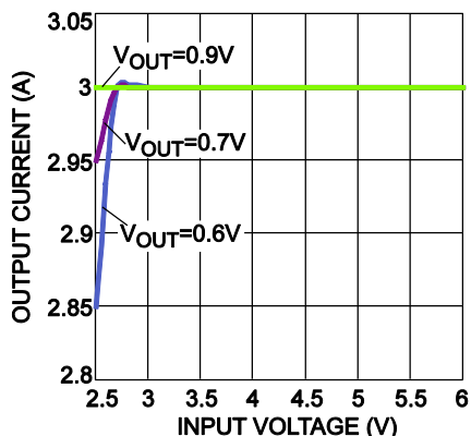
Figure 4: Max I OUT for a Certain Input Voltage
