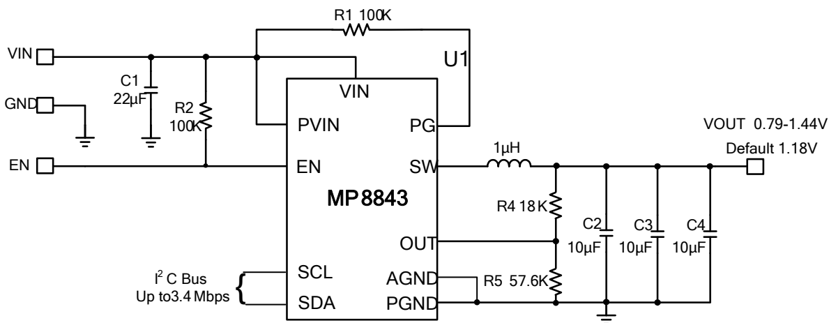
Figure 7: V OUT Range Extended by External Feedback Resistor Network
