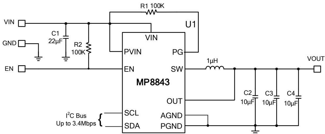
Figure 6: V OUT Range Adjusted from 0.6V to 1.1V
