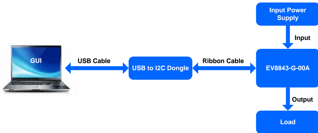
Figure 1. EVKT-8843 Evaluation Kit Setup
