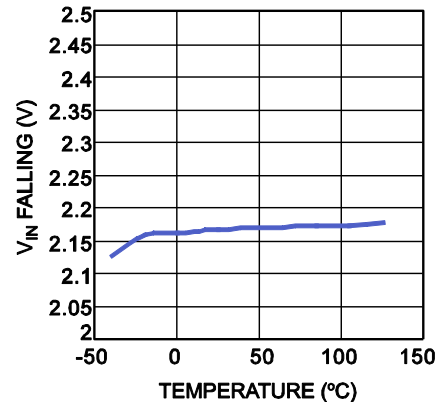
V_{IN} Falling vs. Temperature
