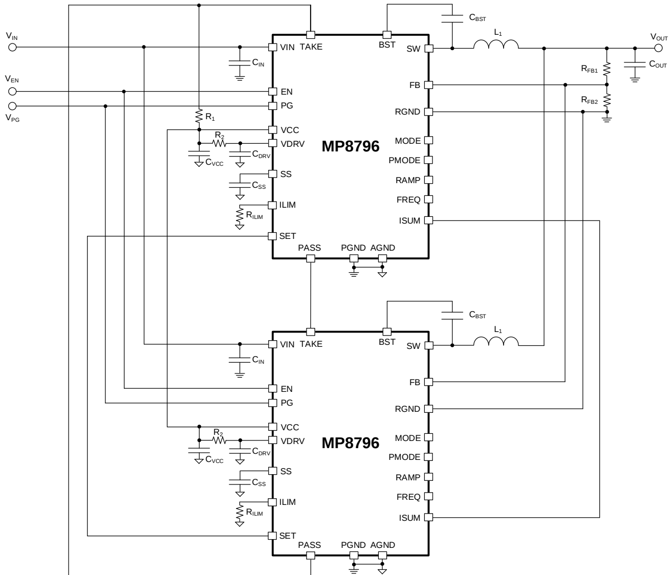
Figure 2: Dual-Phase Operation
