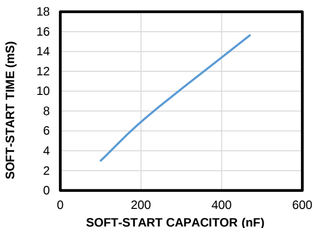
Soft-Start Time vs. Soft-Start Capacitance
