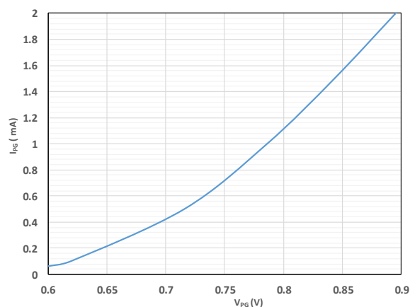
Figure 8: V_{PG} vs. I_{PG}
