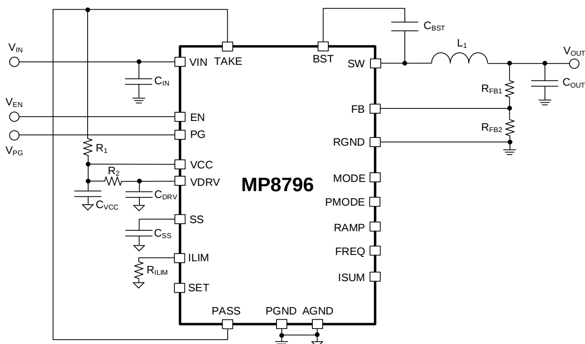
Figure 1: Single-Phase Operation
