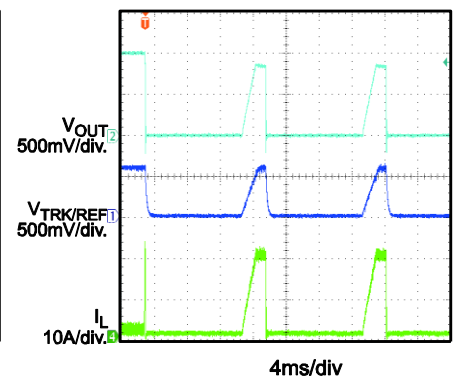
Over-Current
