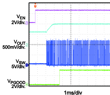
Pre-bias Start-Up
