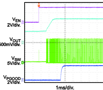
Pre-Biased Start-Up
