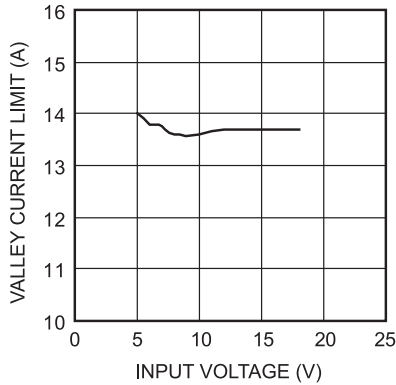
Valley Current Limit vs. Input Voltage
