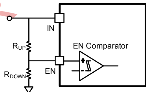
Figure 9—Adjustable UVLO
