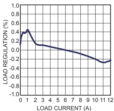
Load Regulation
