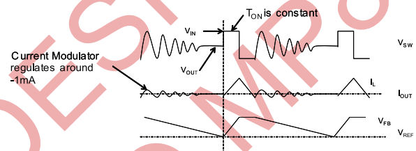
Figure 3: Light-Load Operation
