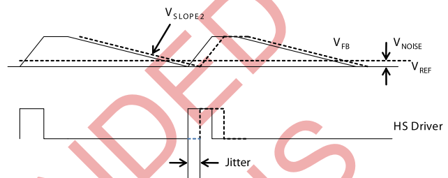
Figure 5: Skip-Mode Jitter
