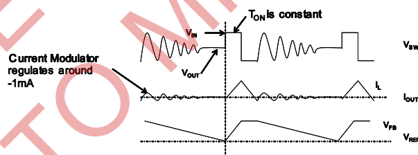
Figure 3: Light-Load Operation
