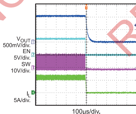
Shutdown Through EN I_{OUT} = 6A
