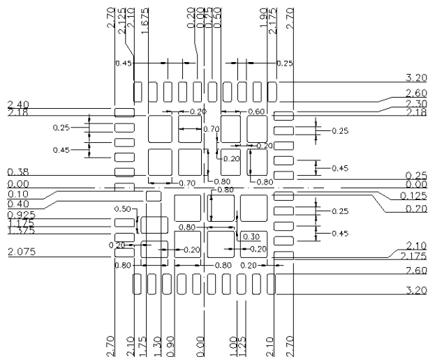
RECOMMENDED STENCIL DESIGN
