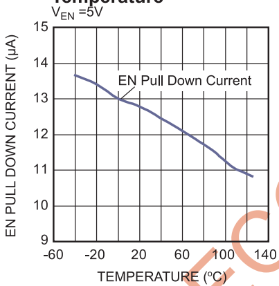
EN Pull Down Current vs. Temperature V_{EN} = 5V
