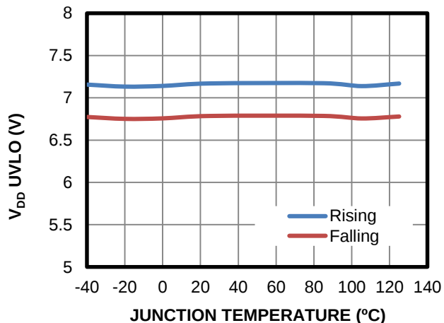
V DD UVLO vs. Junction Temperature
