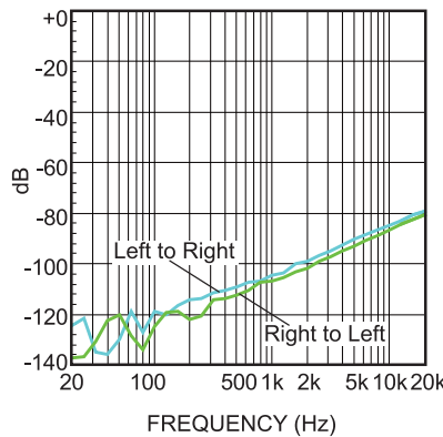
Cross Talk (12V, 8Ω+66μH, P_{OUT}=5W )
