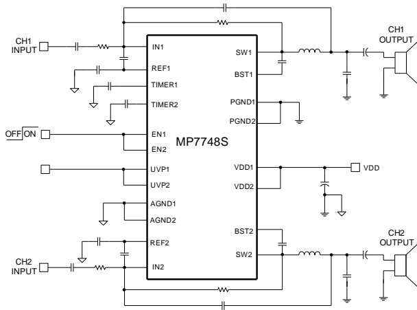
Stereo SE Application Circuit
