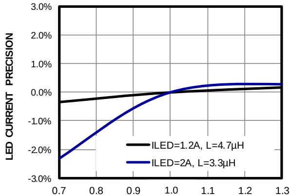
I_{LED} Precision vs. LS-FET Temperature Sense
