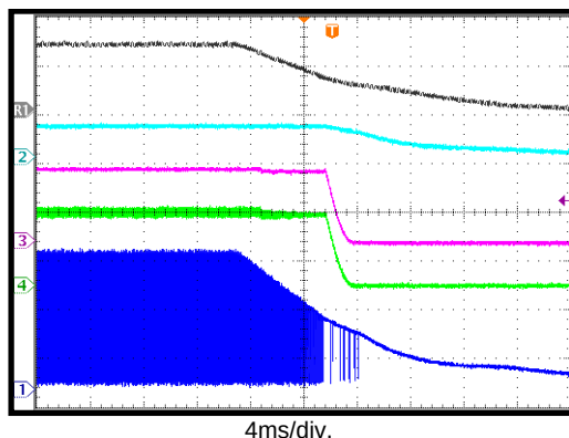
Shutdown through EN/DIM
