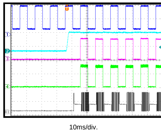
PWM Dimming
