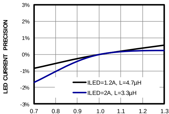
I_{LED} Precision vs. HS-FET Temperature Sense
