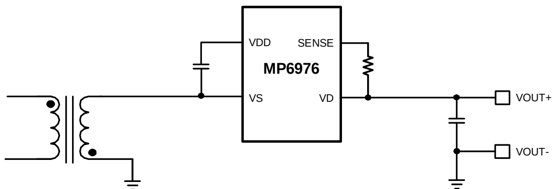
Figure 7: Typical Application Circuit
