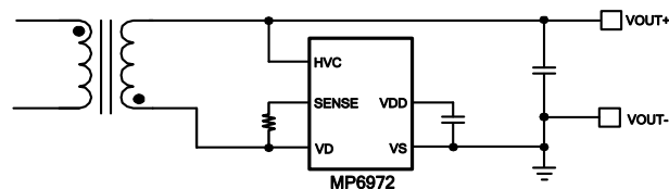
Figure 3: Low-Side Rectification
