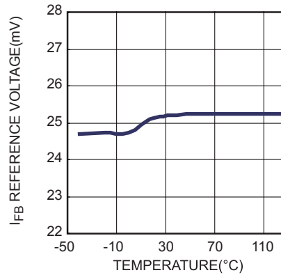
I FB Reference Voltage vs. Temperature
